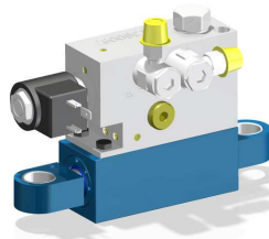
Control valve cylinder with 4/2 directional valve and counterbalance overcenter valves
